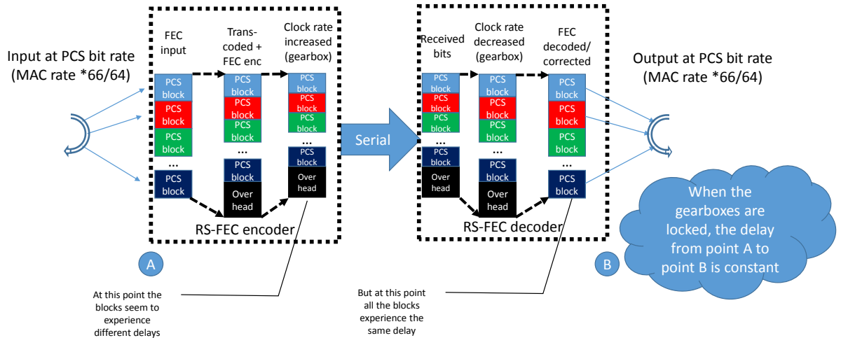
Figure 1: Synchronous FEC encoding and decoding
